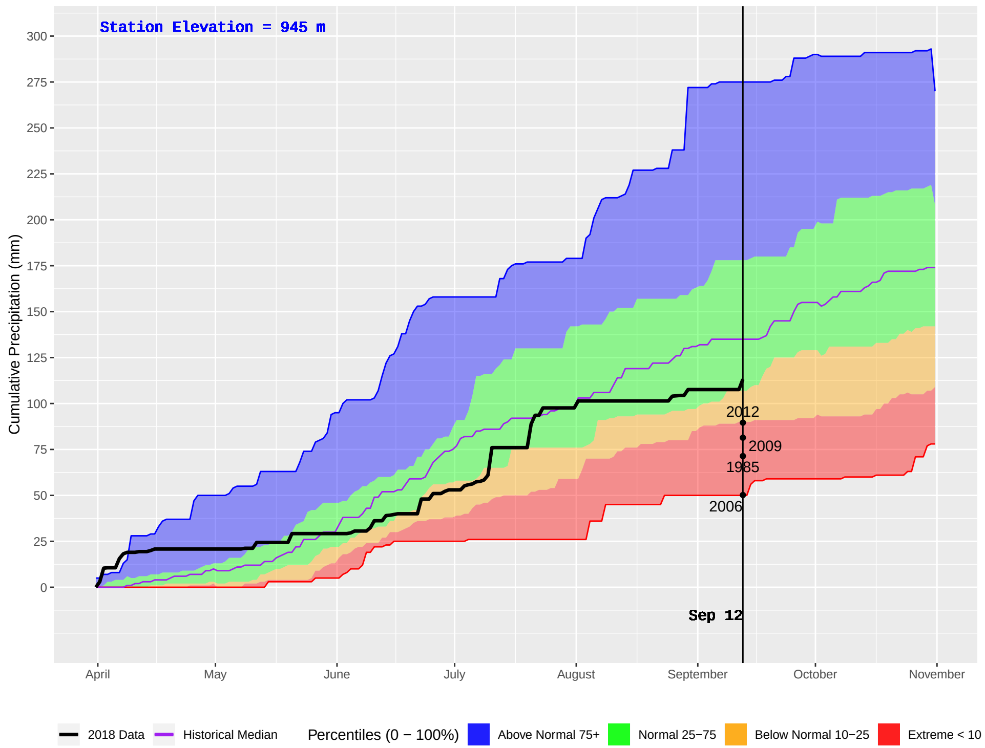
TATLA LAKE HUB (208) : Historical (1980–2016) and Current (2018) Daily Cumulative Precipitation
