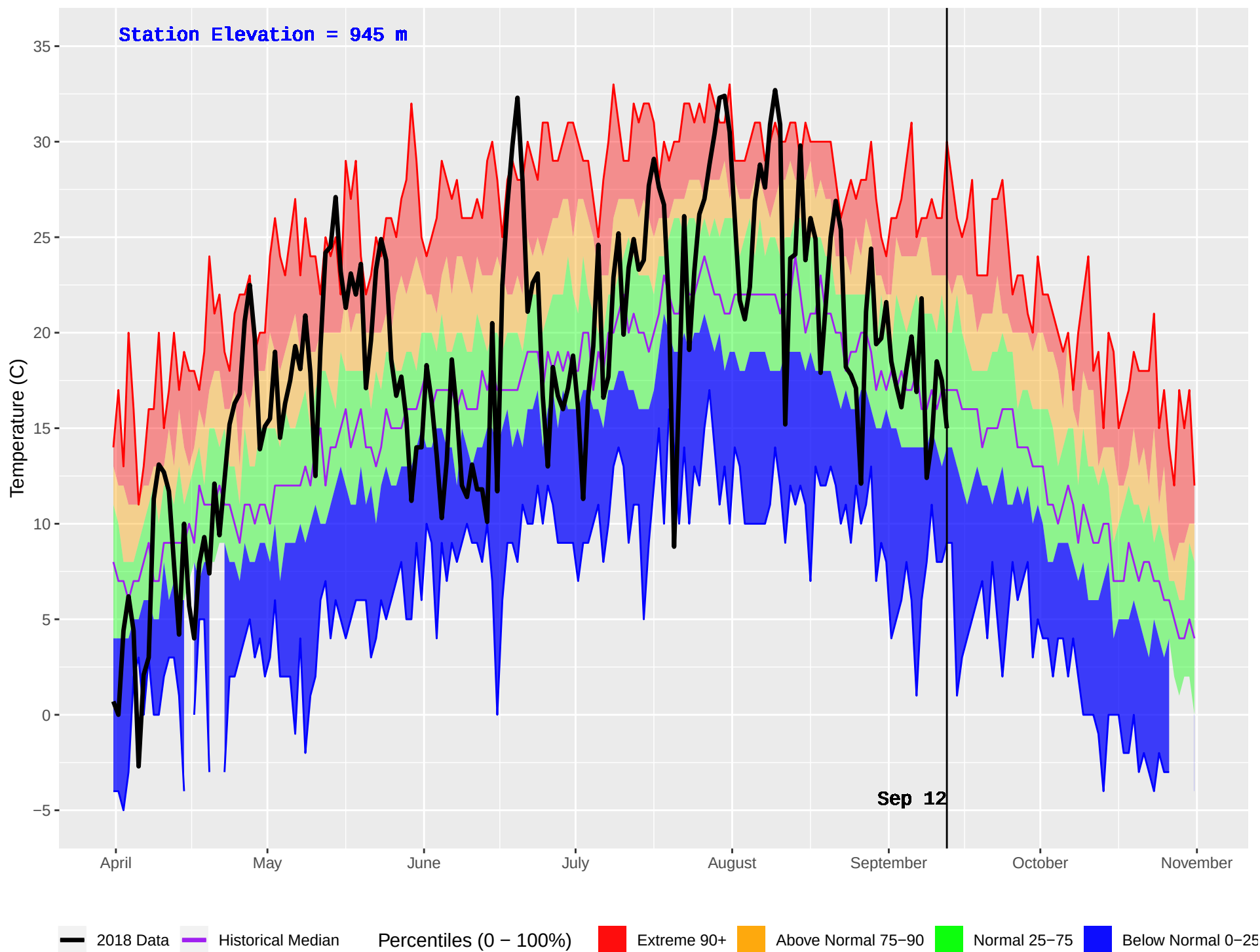
TATLA LAKE HUB (208) : Historical (1980–2016) and Current (2018) Daily Temperature
